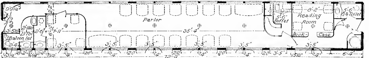
Fig. 178. SECTIONAL PLAN OF BUFFET CAR, PIZON. (Interior view is shown in Fig. 128.)
